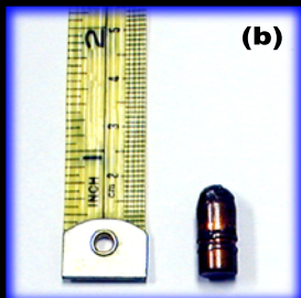
AP Bullets after impacting an X-2+ upgrade insert. (a) 9mm 107gr. KTW @1305 ft./sec. (b) 7.62 x 25mm 85gr. solid steel @1525 ft./sec.
